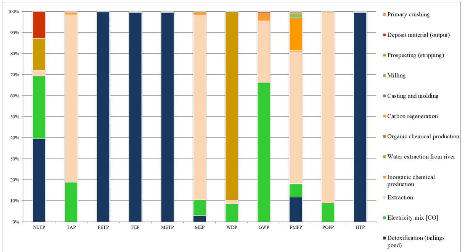
Figure 6 Mid-point indicators for open-pit mining, according to the contribution of the main processes. NLTP : Natural land transformation. TAP : terrestrial acidification. FETP : Freshwater ecotoxicity, FEP : Freshwater eutrophication, METP : Marine ecotoxicity, MEP : Marine eutrophication, GWP : Climate change, POFP : Photochemical oxidant formation, PMFP : Particulate matter formation, WDP : Water depletion, HTP : Human toxicity
