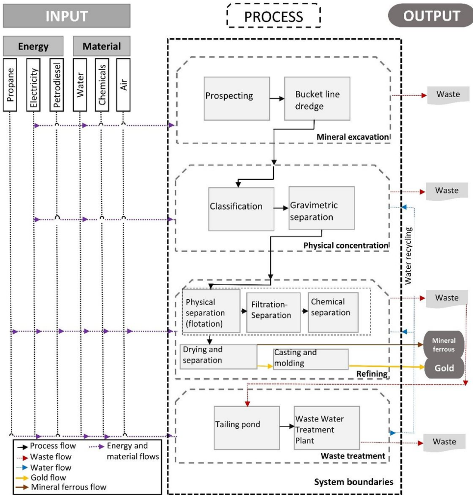
Figure 2 Flow diagram of alluvial mining process from stripping to casting and molding.
