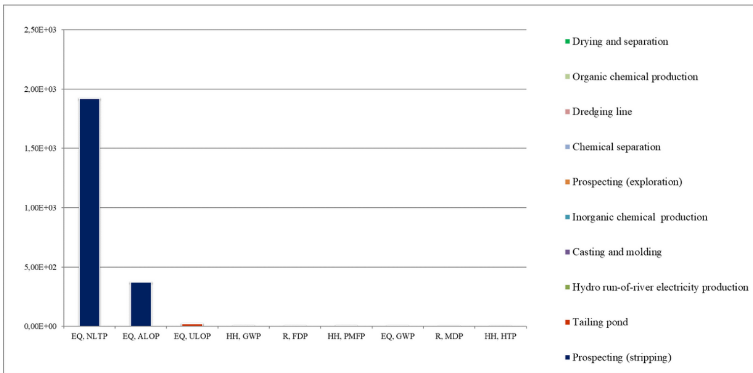
Figure 9 Environmental performance of alluvial mining under end-point indicators, according to the contribution of each process. HH: Human health, R: Resources, EQ: Ecosystem Quality, NLTP: Natural land transformation, ALOP: Agricultural land occupation, ULOP: Urban land occupation, GWP: Climate change, FDP: Fossil depletion, PMFP: Particulate matter formation, MDP: Metal depletion, HTP: Human toxicity
