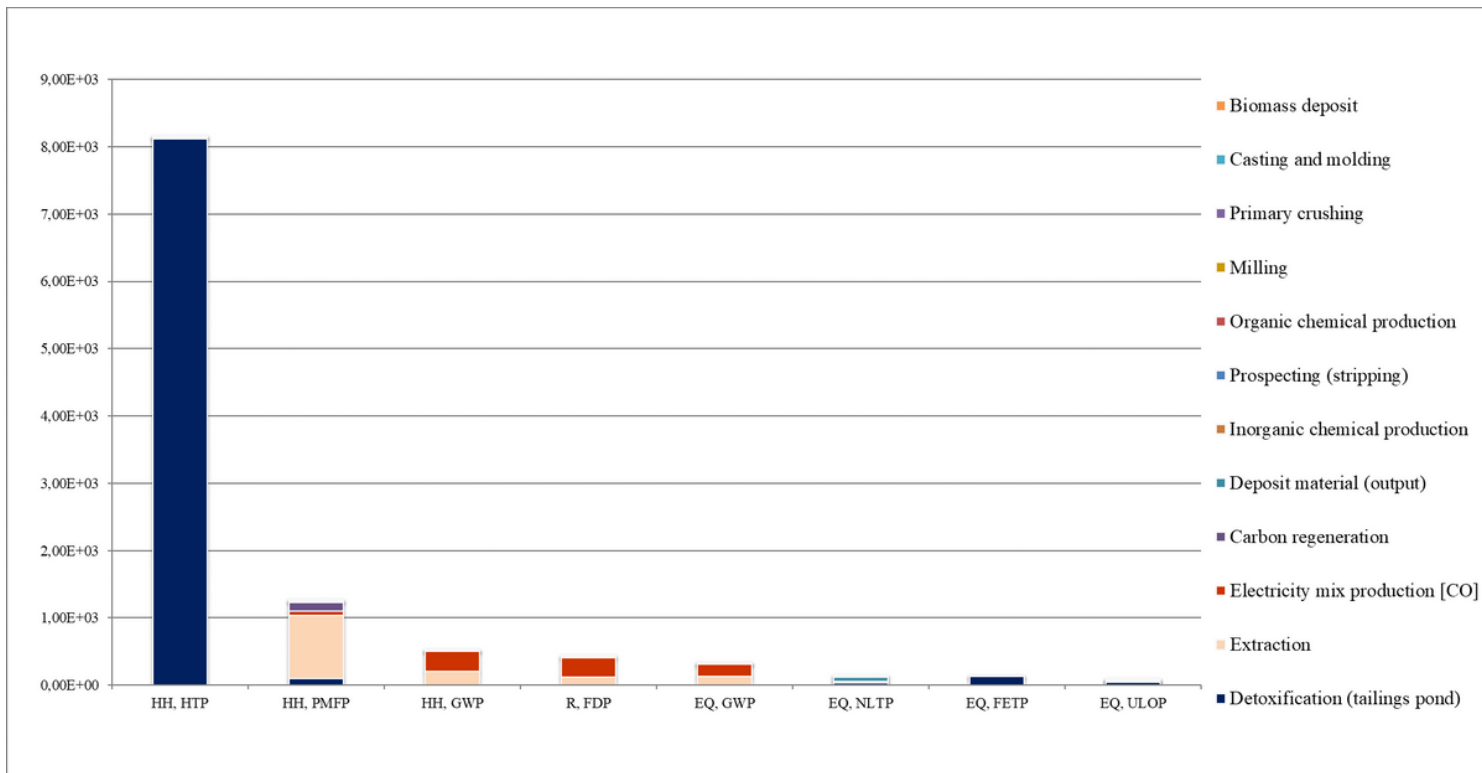
Figure 8 Environmental performance of open-pit mining under end-point indicators, according to the contribution of each process. HH: Human Health, R: Resources, EQ: Ecosystem Quality, HTP: Human toxicity, PMFP: Particulate matter formation, GWP: Climate change, FDP: Fossil depletion, NLTP: Natural land transformation, FETP: Freshwater ecotoxicity, ULOP: Urban land occupation
